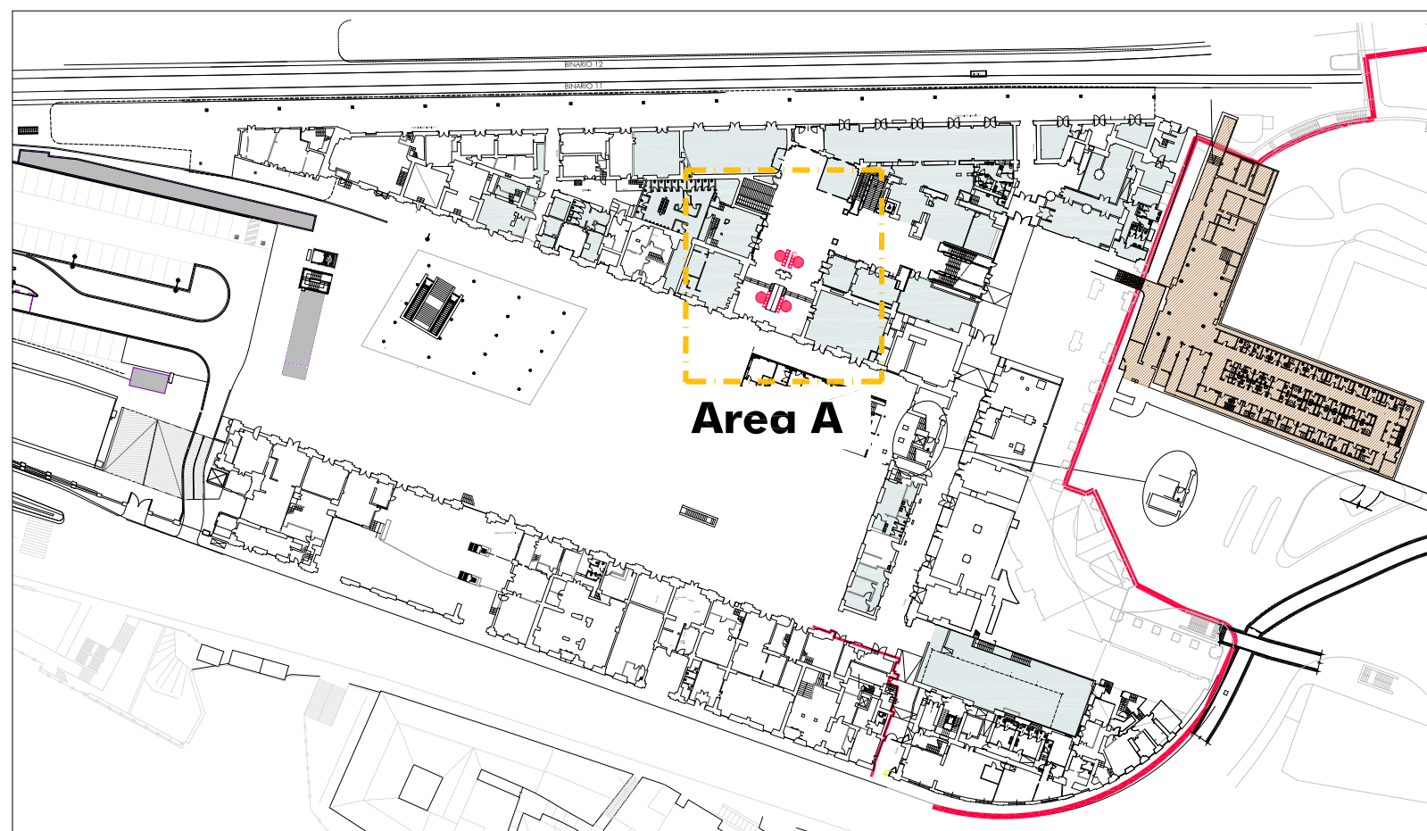
Keyplan - Piano Ferro
