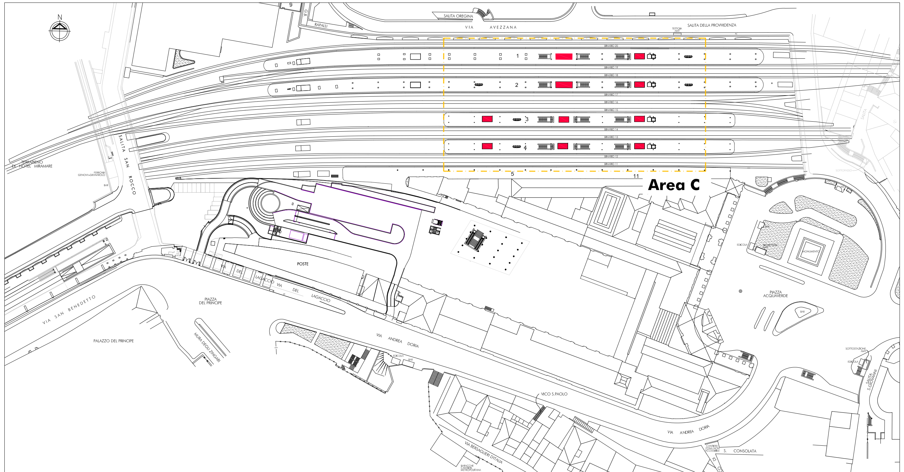
Keyplan - Piano Ferro Banchine Binari
