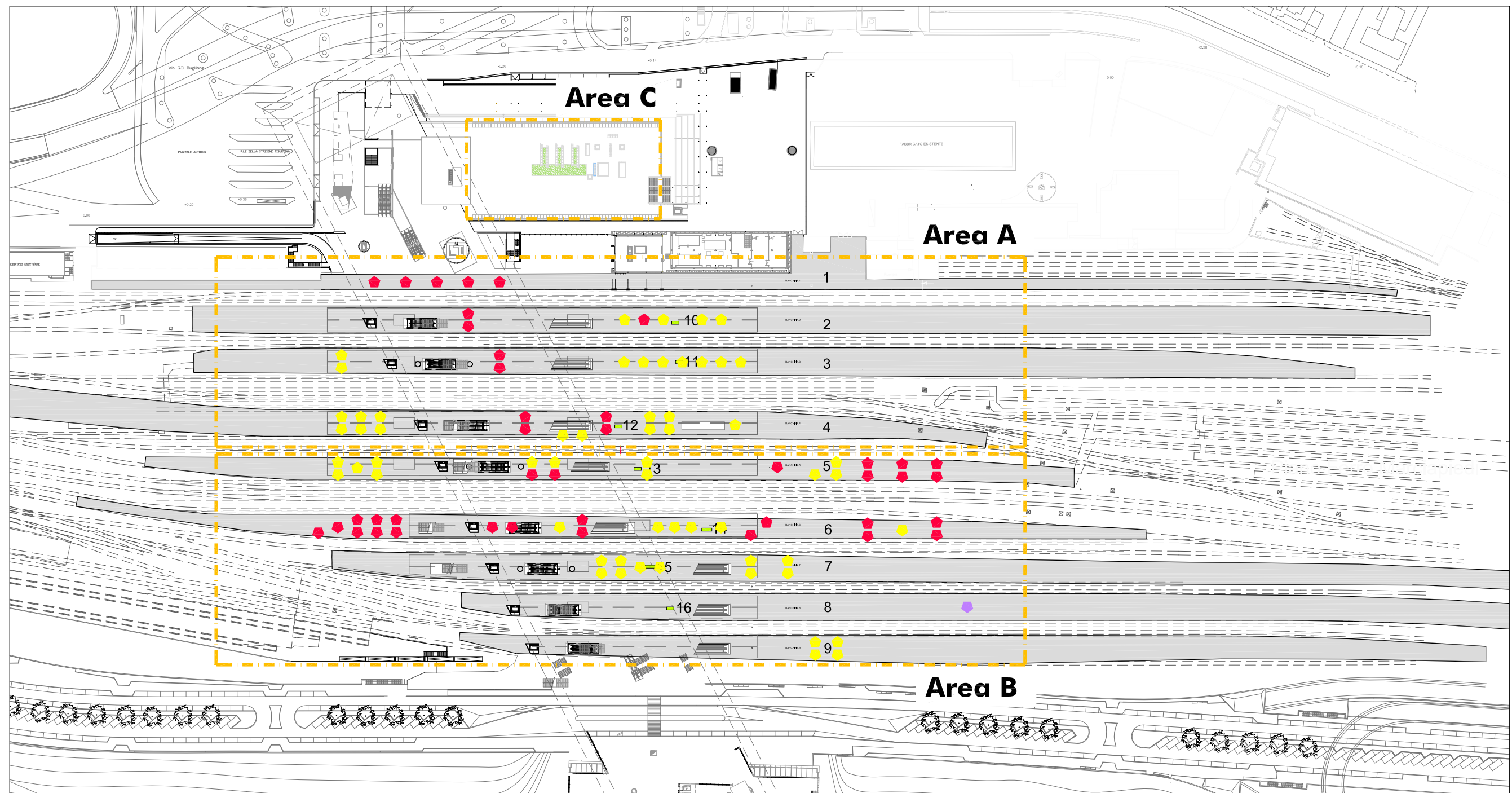
KEYPLAN
