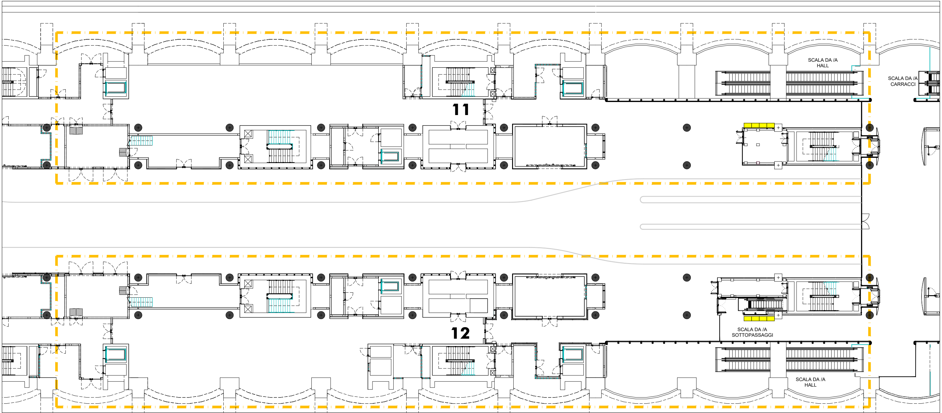
AREA 11-12 : Assi 20-29
